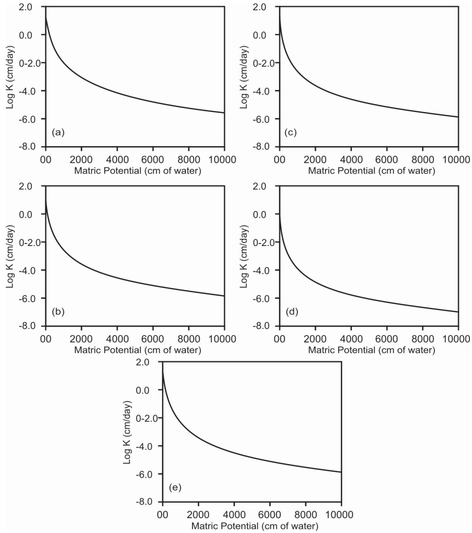
Figure 3. Predicted hydraulic conductivity (log) plotted against matric potential for (a) Jhakkar soil series (b) Matli Soil Series (c) Miani soil series (d) Sarhad soil series and (e) Sultanpur soil series.
